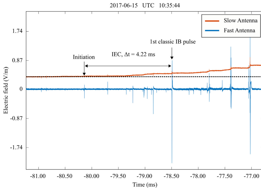
Fig. 4. Example of an IEC (physics sign convention) and the first classical IB pulse for a –CG flash (within reversal distance) captured by wideband fast and slow antenna systems in Malacca at 10:35:44 UTC on June 15th 2017.
