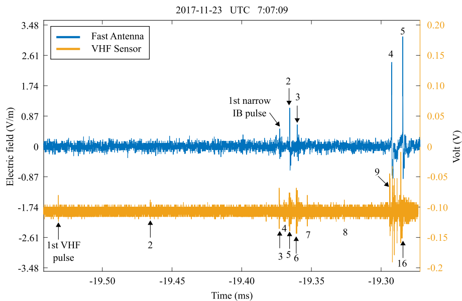
Fig. 11. Plot of VHF pulses and narrow IB pulses for the first normal IC flash (Nov_67). Note that the first two VHF pulses were detected before the first narrow IB pulse and five VHF pulses were coincident with all five narrow IB pulses.
