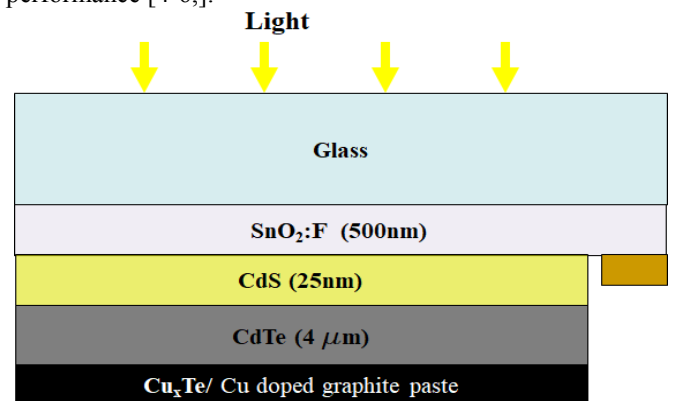
Fig. 1 Structure of CdTe Base cell [13]
