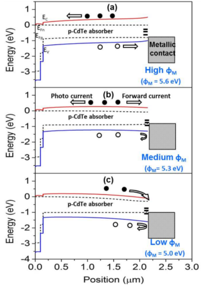
Fig. 3 Band diagram of CdTe cell with different metal work functions [2]
